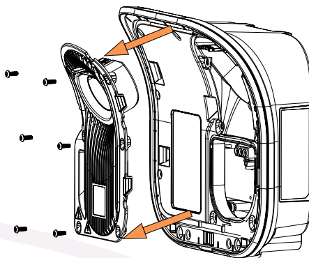
Charging Connector Holder Wiring Window
