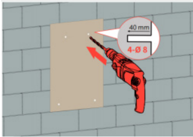
Mark mounting hole
